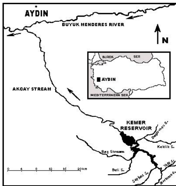
Figure 1. The map of Kemer reservoir and Akçay stream
