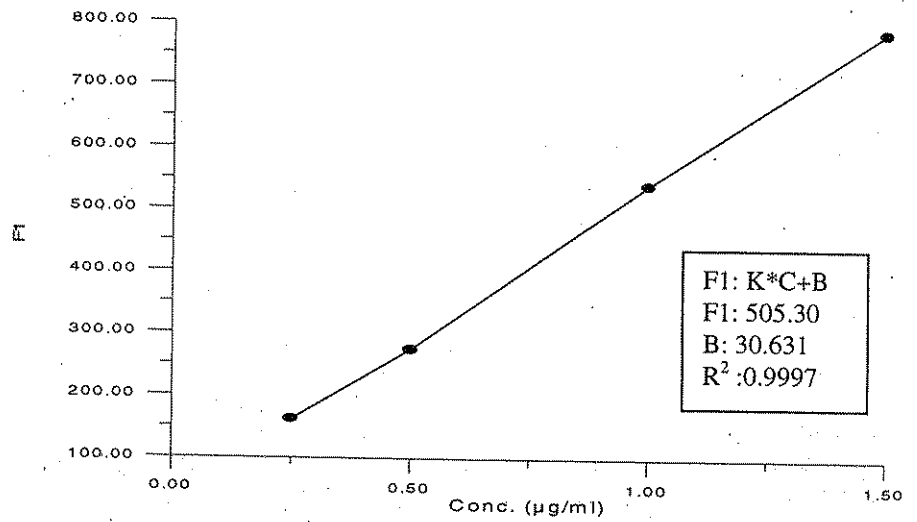
Fig. 3. Standard curve of Iranian crude oil
