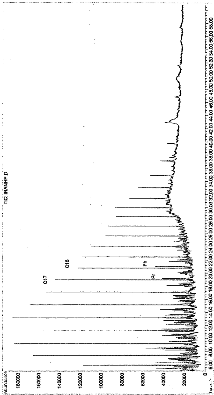
Fig.5. GC/MS Chromatogram of Iranian crude oil
